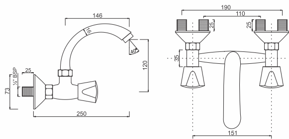
Sink Mixer with Swinging Spout Wall Mounted Cat. No.: 220923
